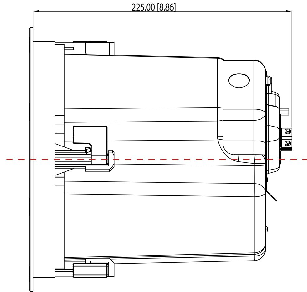
MOUNTING DEPTH
