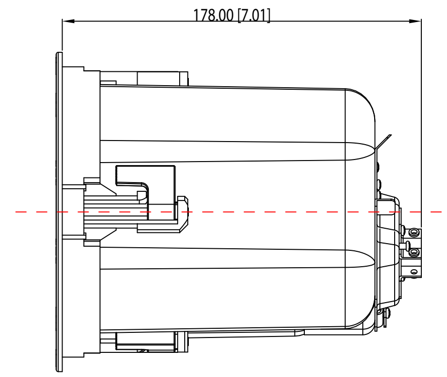
MOUNTING DEPTH
